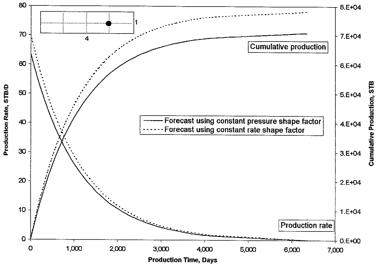
Fig. 3 - Over estimating well productivity when using constant rate shape factors to forecast the production of wells producing at constant pressure.
