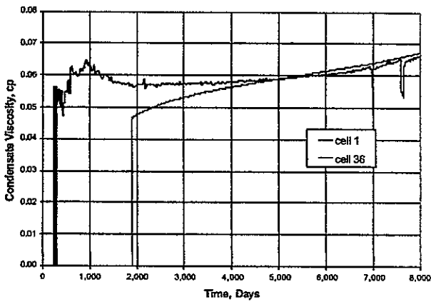
Fig. 10 - Reservoir condensate viscosity
