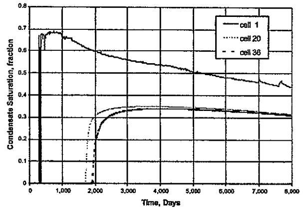
Fig. 6 - Reservoir condensate saturation versus time
