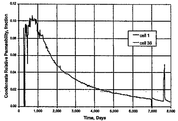
Fig. 7 - Reservoir condensate relative permeability
