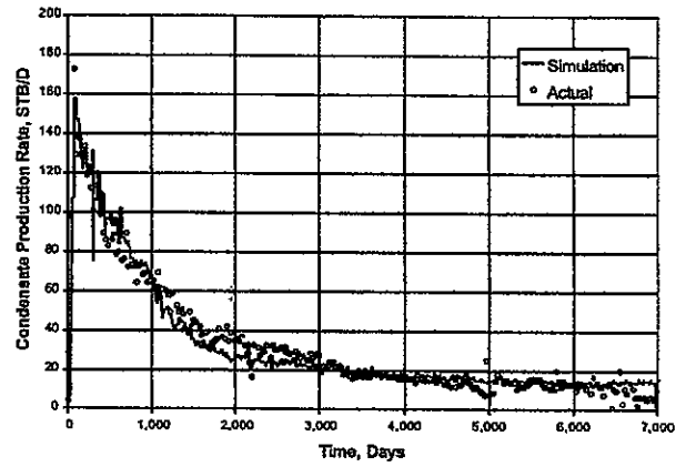
Fig. 5 - History match of condensate production rate
