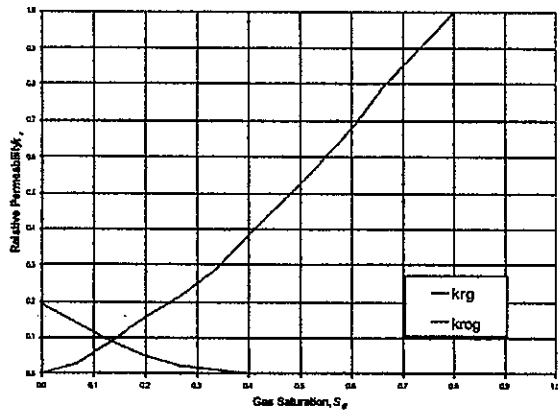
Fig. 4 - Relative permeability curves used in simulation model
