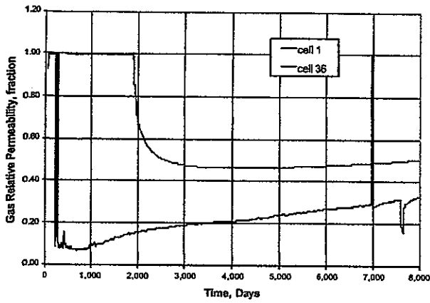
Fig. 8 - Reservoir gas relative permeability
