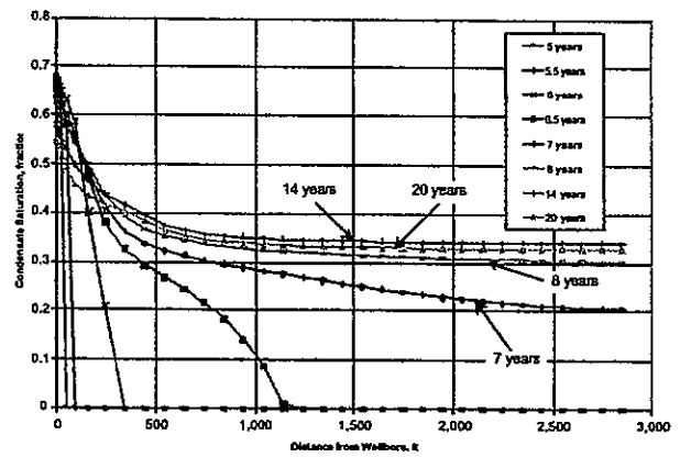
Fig. 12 - Condensate saturation profile change with time
