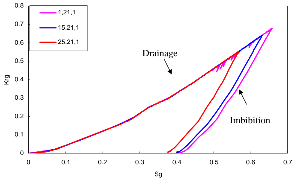
Fig. 5.11. – Illustration of the Drainage Relative Permeability Curve (top) and the Family of Imbibition Curves Calculated for Various Gridblocks in the IMEX Simulator.
