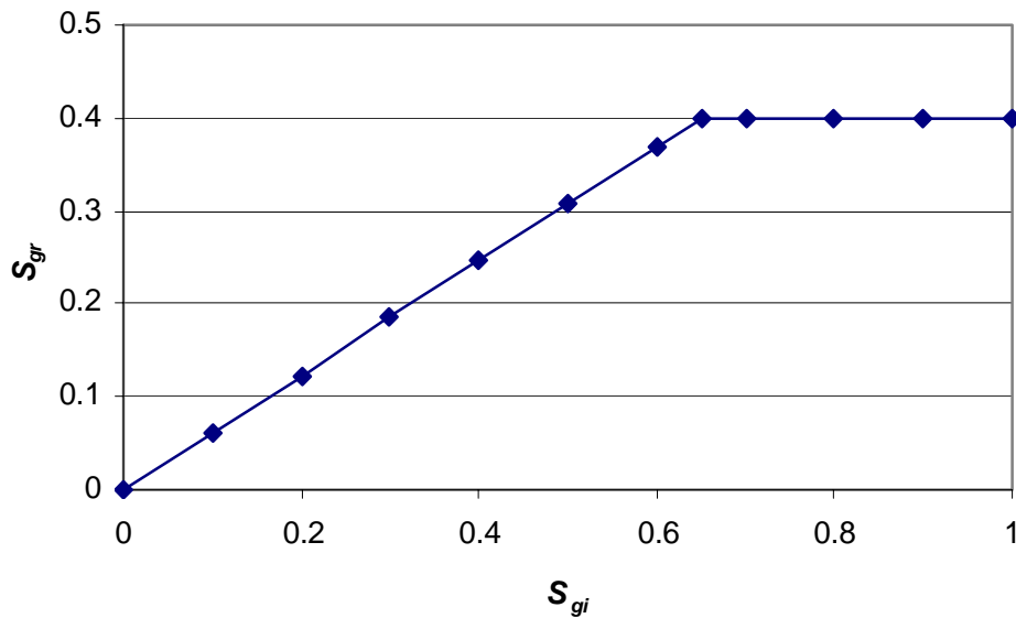
Fig. 5.8 - Theoretical S_{gr} vs S_{gi} Relationship by Aissaoui.
