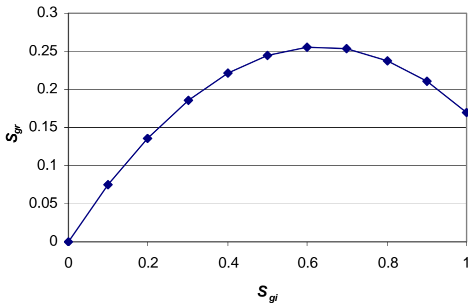
Fig. 5.3 – Theoretical S_{gr} vs S_{gi} relationship of Agarwal.
