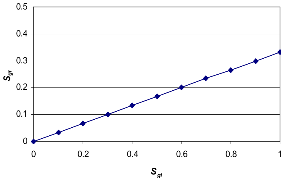
Fig 5.6- Theoretical S_{gr} vs S_{gi} Relationship Proposed by Kleppe
