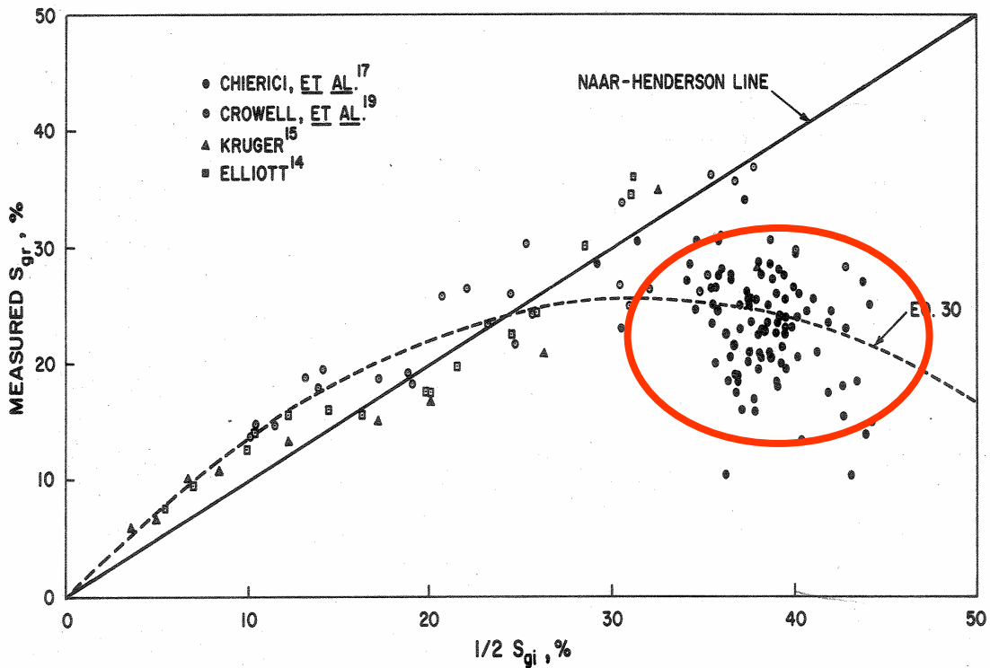
Fig.5.4- Measured S_{gr} vs. Naar Line for the Consolidated Sandstone (Agarwal's dissertation).
